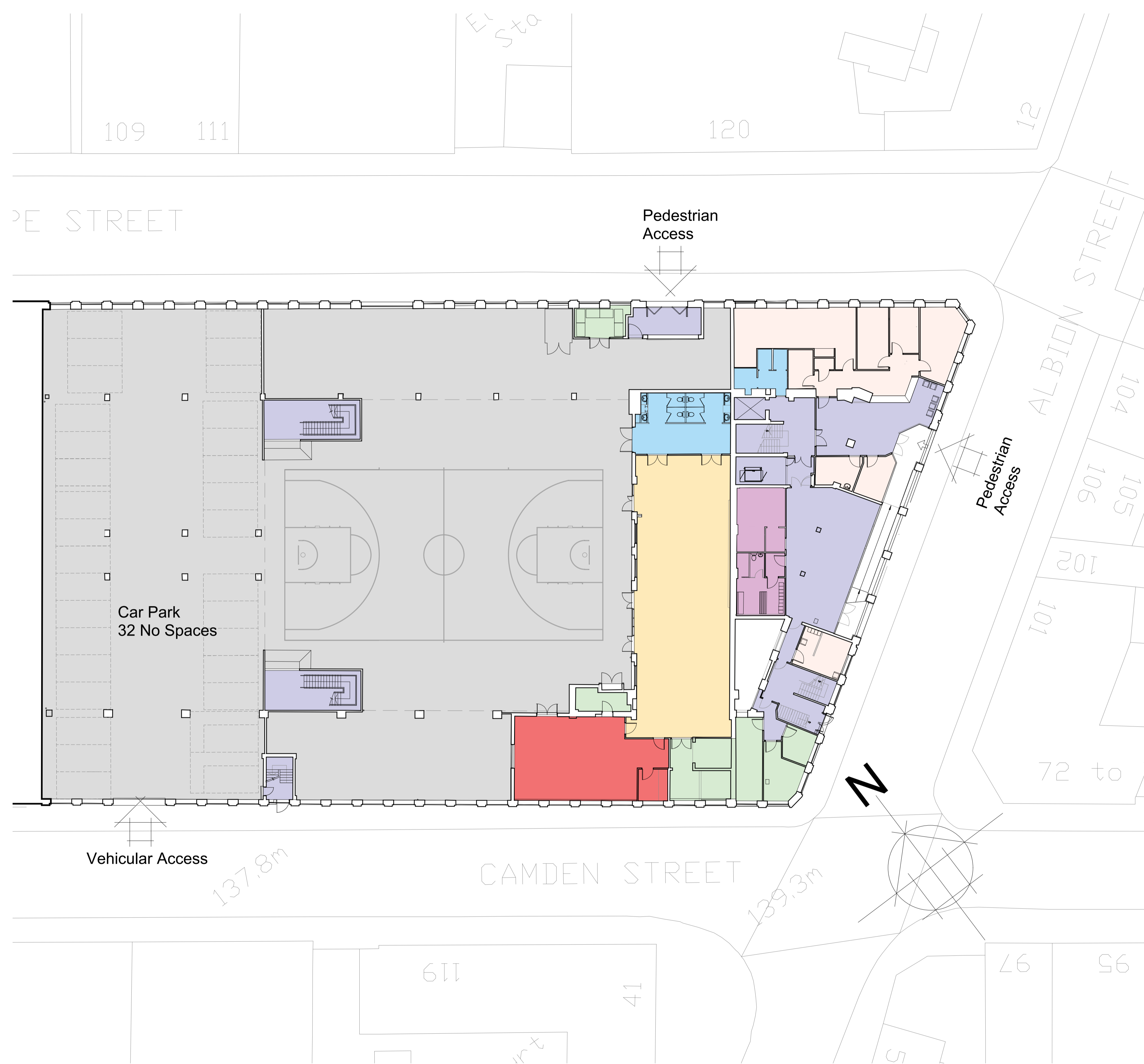
2 BLOCK PLAN Scale 1: 200
